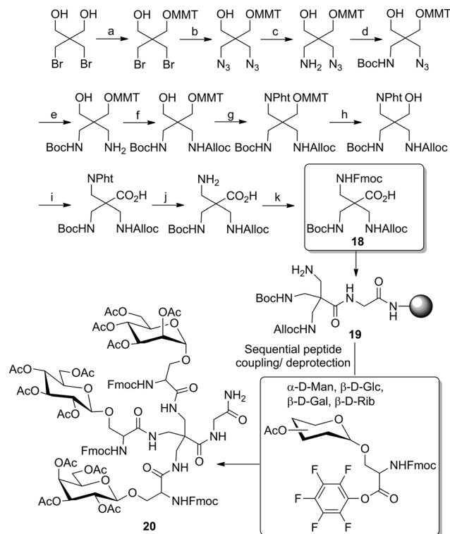
Scheme 2 Solid phase-supported synthesis of a trivalent heteroglycocluster based on a pentaerythritol scaffold. Reagents and conditions: (a) MMT-Cl, pyridine, 94%; (b) \text{NaN}_3 , LiCl, DMF, pyridine, 84%; (c) \text{NaBH}_4 , \text{HS}(\text{CH}_2)_3\text{SH} , \text{Et}_3\text{N} , i PrOH, 45%; (d) \text{Boc}_2\text{O} , NaOH, MeCN, 99%; (e) \text{PPh}_3 , aq. \text{NH}_3 , 82%; (f) AllocCl, \text{Et}_3\text{N} , dioxane, 78%; (g) phthalimide, \text{PPh}_3 , DEAD, THF, 66%; (h) \text{I}_2 , MeOH, DCM, 72%; (i) \text{CrO}_3/\text{H}_2\text{SO}_4 , \text{H}_2\text{O} , acetone, 54%; (j) \text{NH}_2\text{NH}_2 , allyl alcohol, DMF, dioxane, 71%; (k) FmocCl, \text{K}_2\text{CO}_3 , \text{H}_2\text{O} , MeCN, 70%.
