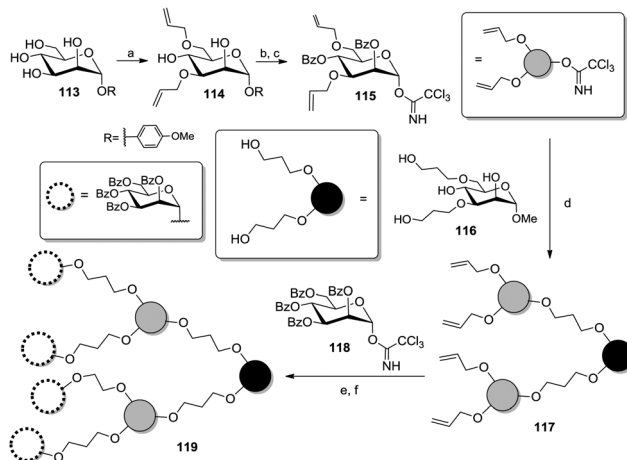
Scheme 17 Regioselective di-allylation of a mannose scaffold for the construction of a dendrimer. Reagents and conditions: (a) (i) bis(tributyltin)oxide, toluene, reflux; (ii) AllBr, TBABr, 80 °C, 51%; (b) BzCl, pyridine, 0 °C to rt, quant.; (c) (i) CAN, MeCN/H 2 O (4 : 1), 0 °C to rt; (ii) trichloroacetonitrile, DBU, DCM, 0 °C to rt, 53% over two steps; (d) TMSOTf, DCM, rt, 79%; (e) (i) 9-BBN, THF, reflux; (ii) 3M NaOAc (aq.), H 2 O 2 (30%), 0 °C to rt, 40%; (f) TMSOTf, DCM, rt, 54%.
